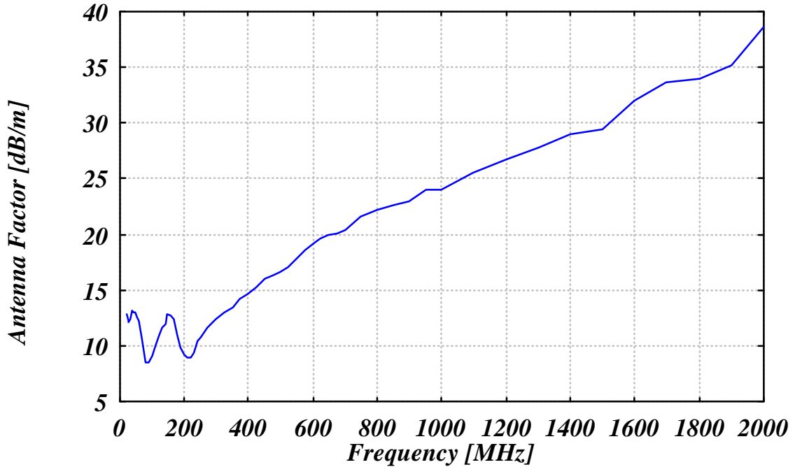
Antenna Factor
