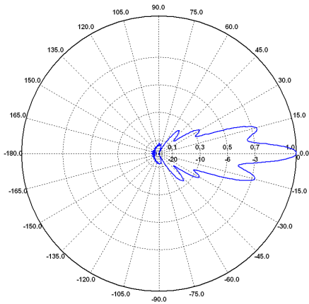
E-Ebene / E-Plane 10 GHz
