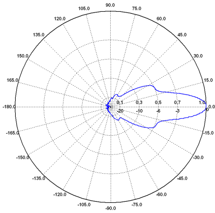
E-Ebene / E-Plane 6 GHz
