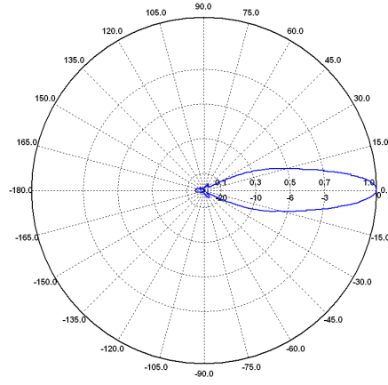
H-Ebene / H-Plane 8 GHz
