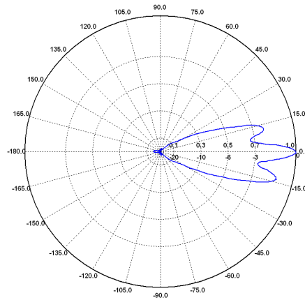
H-Ebene / H-Plane 10 GHz
