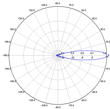
H-Ebene / H-Plane 9 GHz
