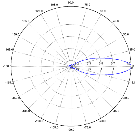
H-Ebene / H-Plane 7 GHz
