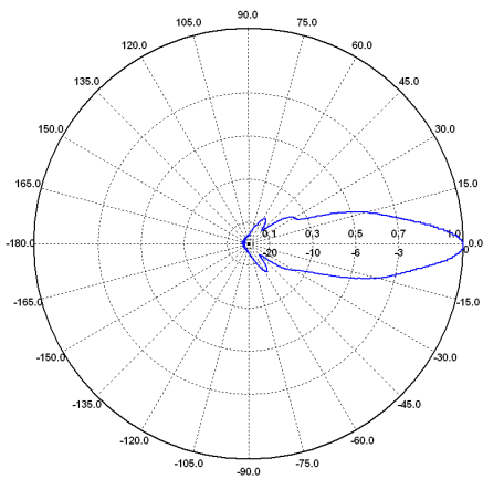
E-Ebene / E-Plane 9 GHz
