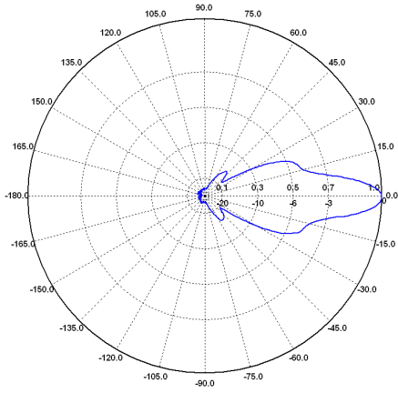
E-Ebene / E-Plane 7 GHz
