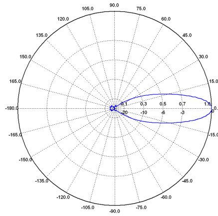
H-Ebene / H-Plane 6 GHz
